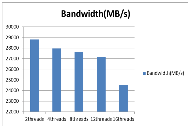
Figure 2 : (Bonnie++) Bandwidth
