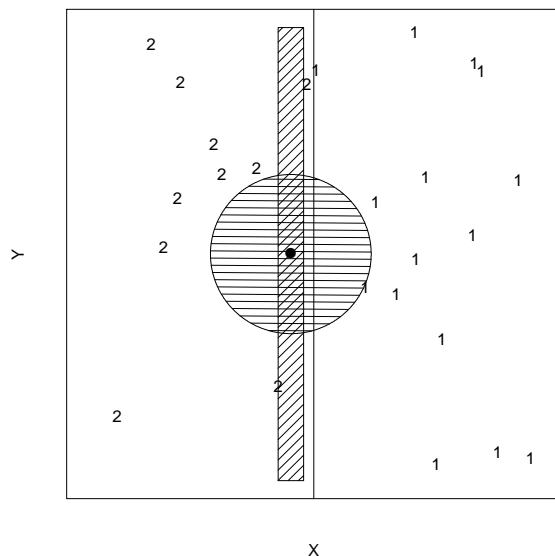
Figure 1: The points are uniform in the cube, with the vertical line separating class 1 and 2. The vertical strip denotes the NN region using only the X coordinate to find the nearest neighbor for the target point (solid dot). The sphere shows the NN region using both coordinates, and we see in this case it has extended into the class 1 region (and found the wrong class in this instance).
