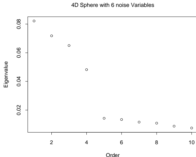
Figure 4: The eigenvalues of the average between matrix for the 4D sphere + 6 noise variable problem. Using these first four dimensions followed by our DANN nearest neighbor routine, we get better performance than 5NN in the real 4D subspace.
