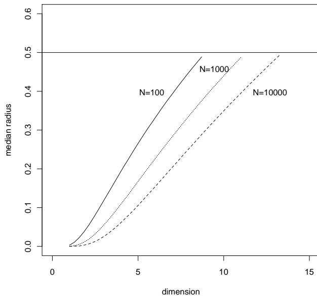
Figure 8: Median radius of a one-nearest neighborhood as a function of dimension and size of training sample.
