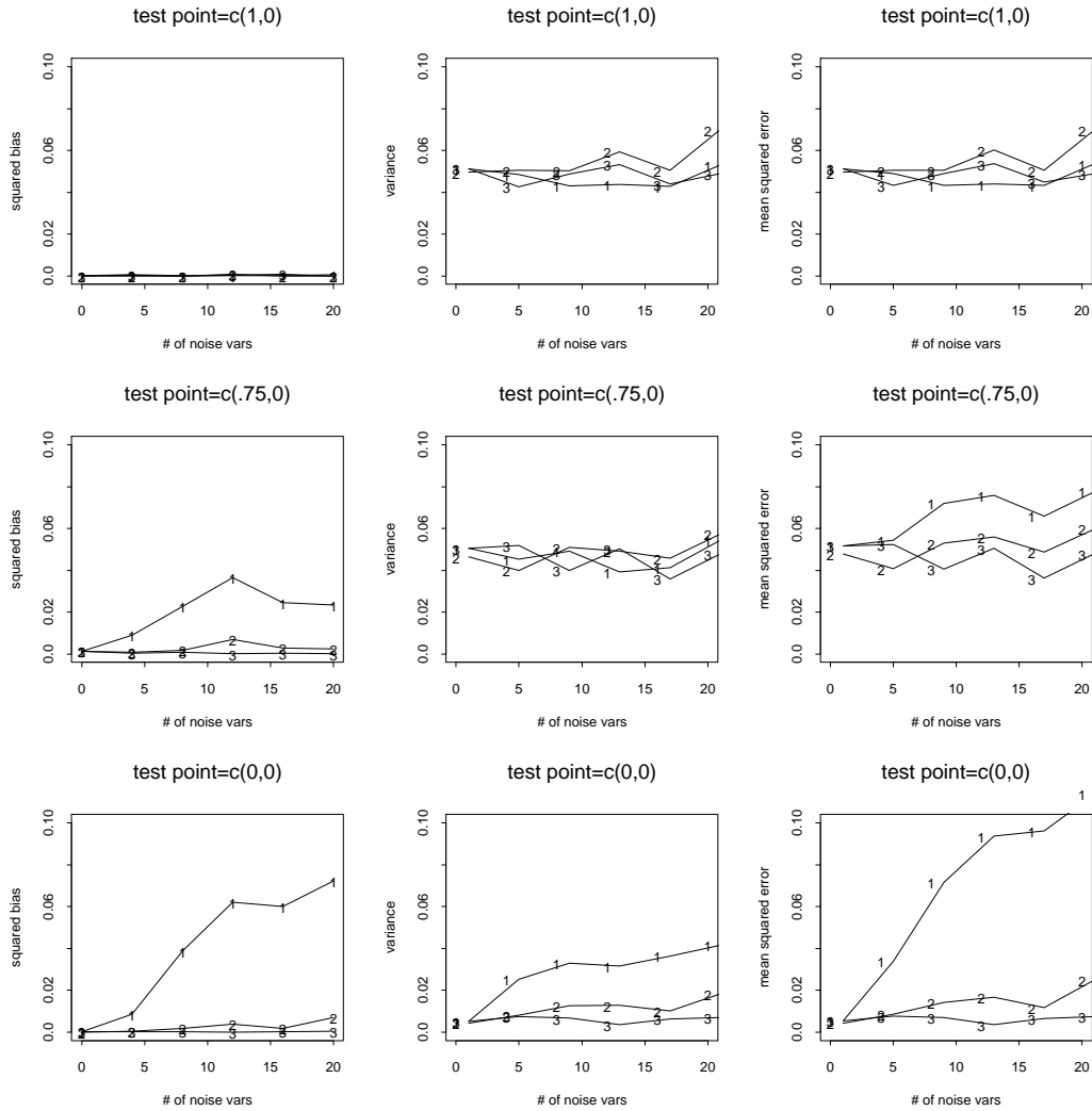
Figure 9: Bias, variance and mean squared error of 5-NN (1), DANN (2) and 5-NN restricted to the first predictors (3). There are two classes with centers (0,0) and (2,0). In the top, middle and bottom rows the prediction is done at (1,0), (.75,0) and (0,0) respectively. The simulation standard errors of the bias and variance estimates are roughly .015 and .003 respectively.
