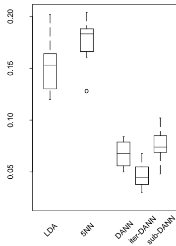
Figure 6: Boxplots of error rates over 20 simulations, second four simulated examples.
