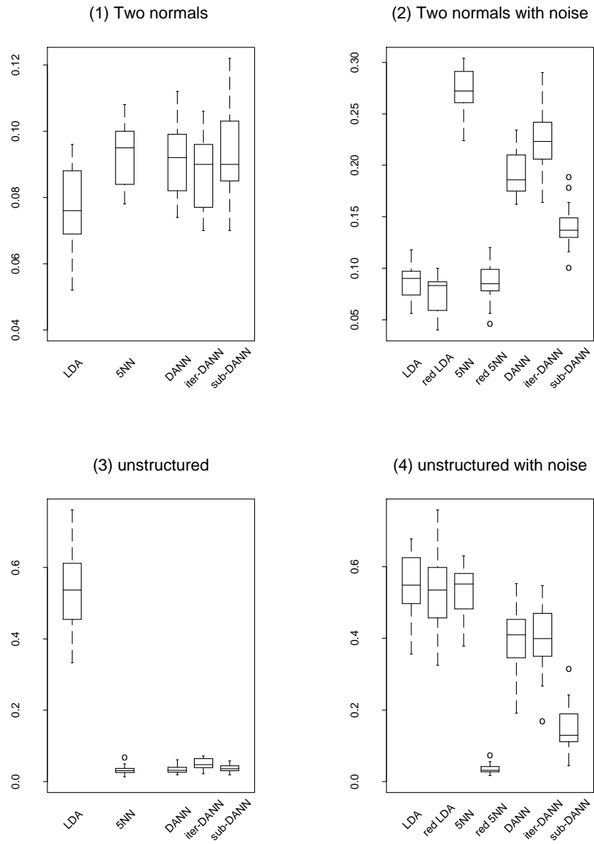
Figure 5: Boxplots of error rates over 20 simulations, first four simulated examples.
