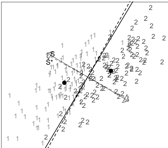
LDA and Local Subspaces --- K = 25
