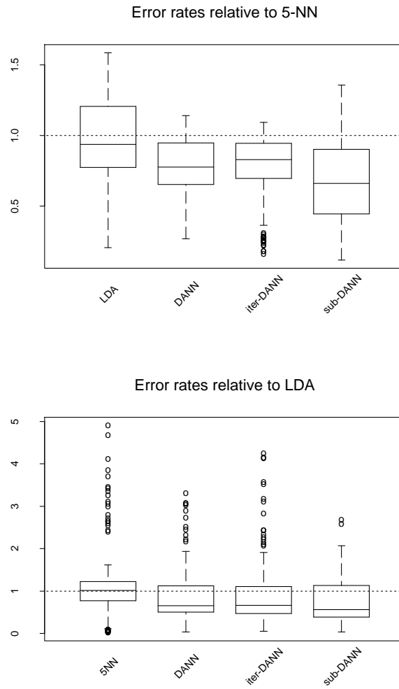
Figure 7: Relative error rates of the methods across the 8 simulated problems. In the top panel the error rate has been divided by the error rate 5-NN, on a simulation by simulation basis. In the bottom panel we have divided by the error rate of LDA.
