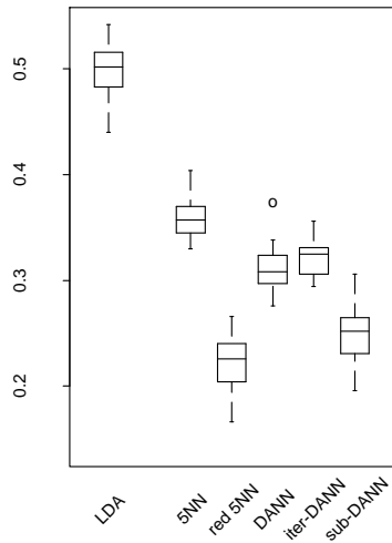
(5) Four dim sphere in ten dim
