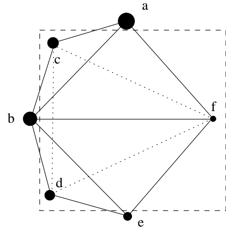
Figure 4: Pattern edges that are not Delaunay edges
