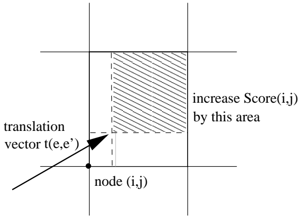
Figure 6: Updating the score for a pair e, e' of similar edges
