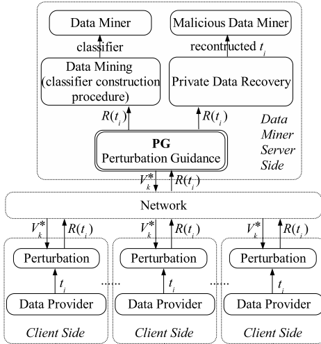
Figure 2: Our New Scheme
