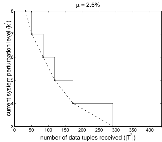
Figure 5: Change of k^* with |T^*|
