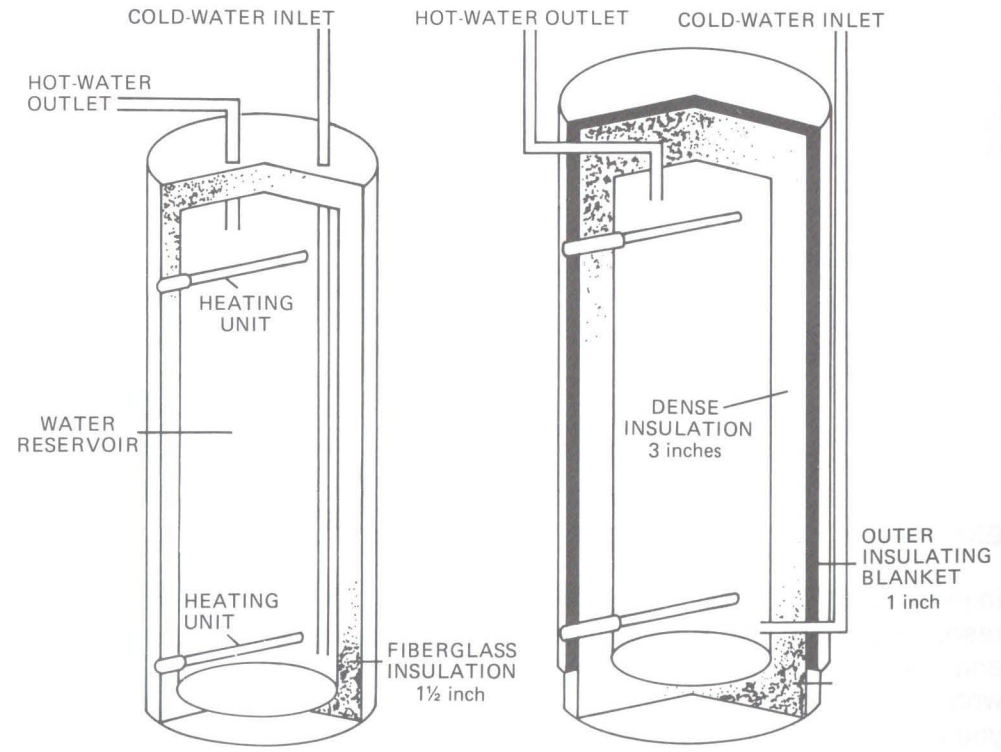
FIGURE 6.6 Conventional and experimental hot water heaters.
