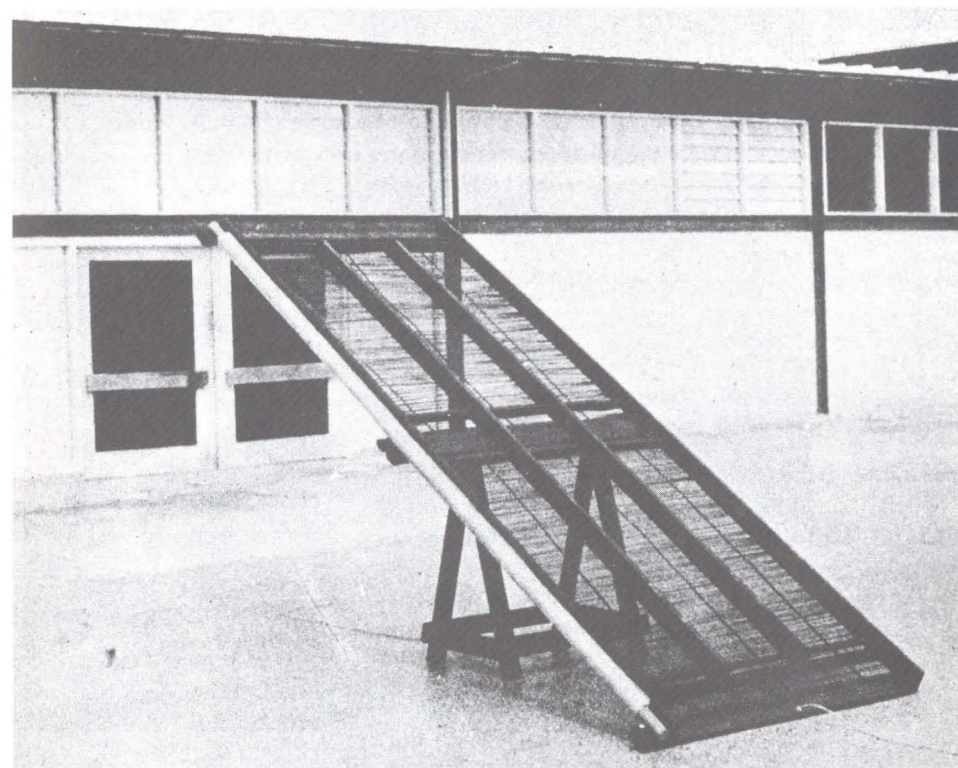
FIGURE 6.2 Solar food dryer.
