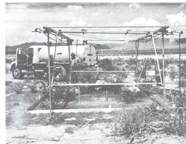
FIGURE 6.3 Rainfall simulator.
