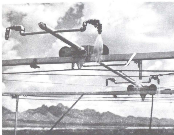
FIGURE 6.4 Spray assembly.
