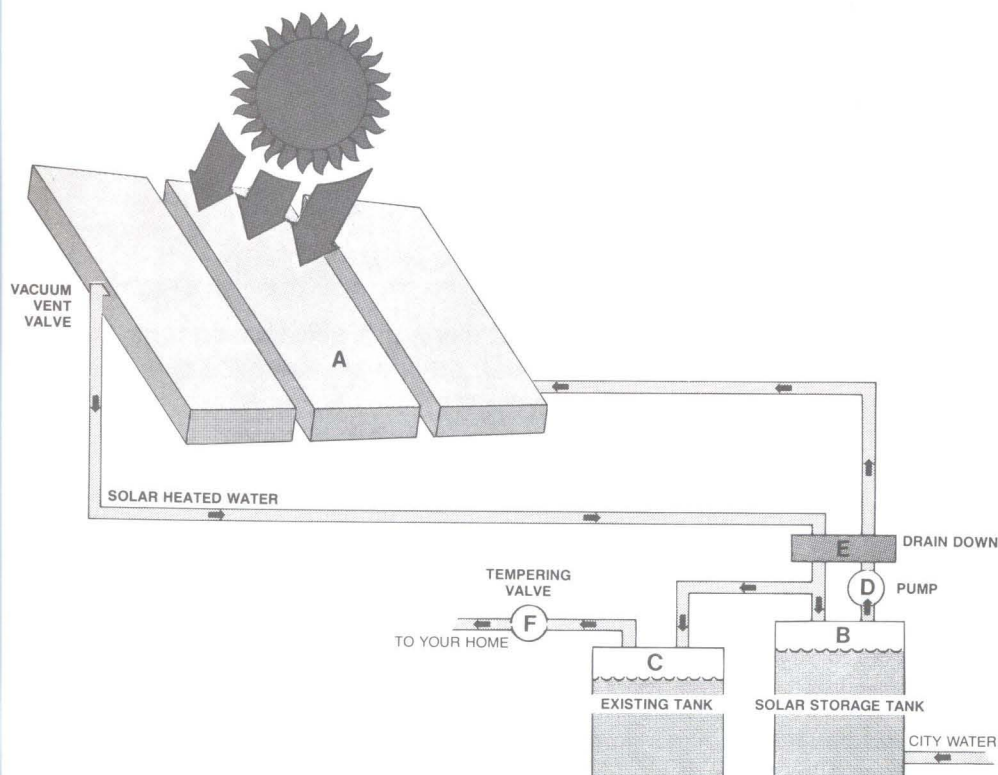
FIGURE 6.5 Solar water heating system.
