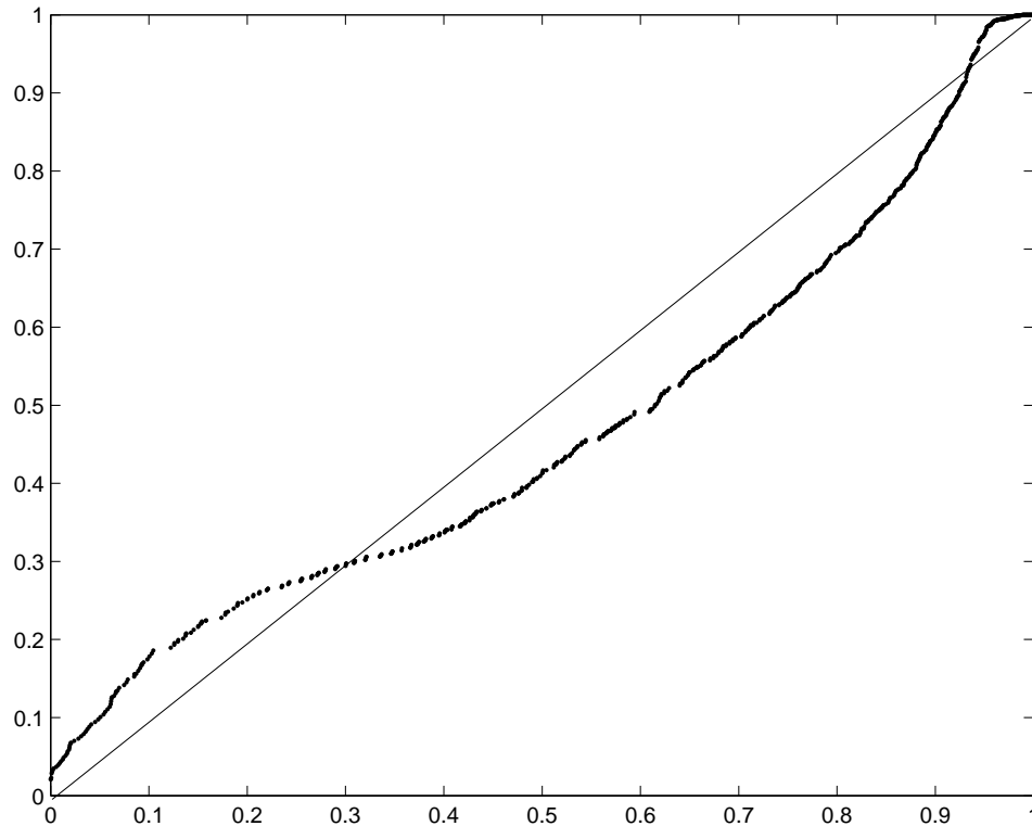
Figure 9: pp-plot.
