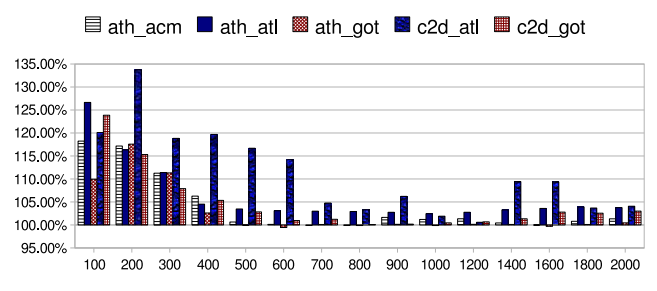
(c) DGETRF (LU) on Athlon-64 and Core2Duo
