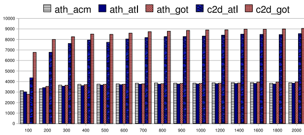
(a) DGEMM (matrix multiply)
