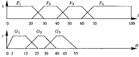
Figure 1. Fuzzy Terms
