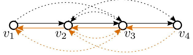
Fig. 1: Example with two concurrent policy updates: at the top update (\pi_1^{(1)}, \pi_2^{(1)}) in black , at the bottom update (\pi_1^{(2)}, \pi_2^{(2)}) in orange . The old policies (\pi_1^{(1)}) and \pi_1^{(2)} are drawn using solid lines , the new policies (\pi_2^{(1)}) and \pi_2^{(2)} using dashed lines . At least one node cannot install both updates simultaneously without creating a loop, and hence, needs two rounds of interactions ( touches ).
