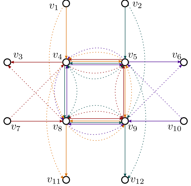
Fig. 2: Construction of a multi-touch lock . Four concurrent policy updates are shown in different colors, the old policies are shown using solid lines, and the new policies are shown using dashed lines of the same color.
