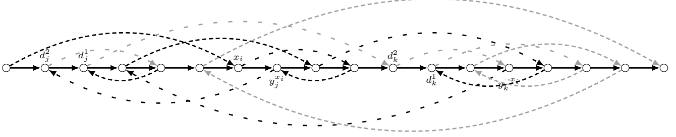
Fig. 9: Complete gadget for a variable. The essential edges of the gadget (presented in Figure 5) are drawn in loosely dashed black , edges of clause gadgets are drawn in loosely dashed grey , edges added to change the node type (described in Section III-B3) are drawn in densely dashed grey and the other edges added to connect the graph are drawn in densely dashed black .
