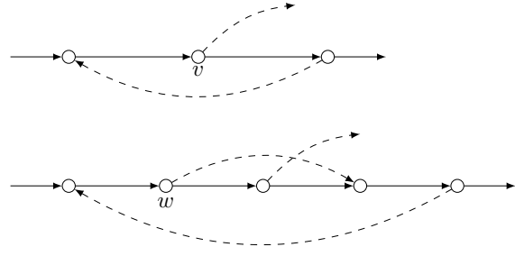
Fig. 4: Examples of FFFF nodes which must be updated in either first or third round.
