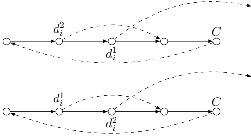
Fig. 6: Gadget for updating clauses in one of the policies.
